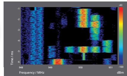
Interference signal
